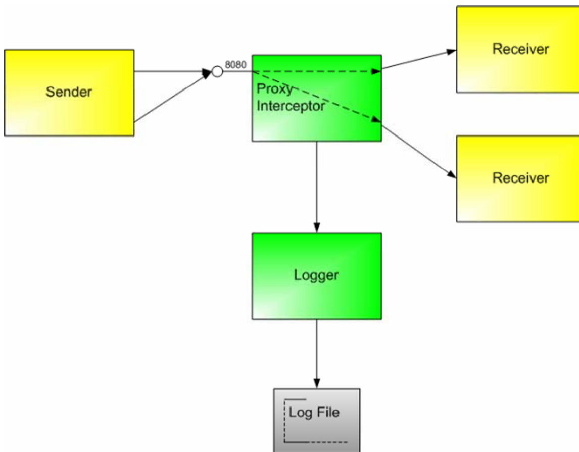
Figure 4. Proxy interceptor
